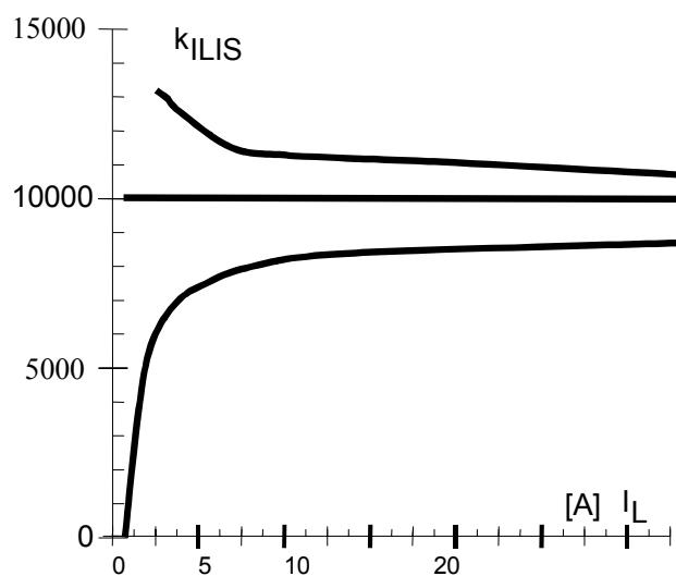
Figure 6b: Current sense ratio 21 :
