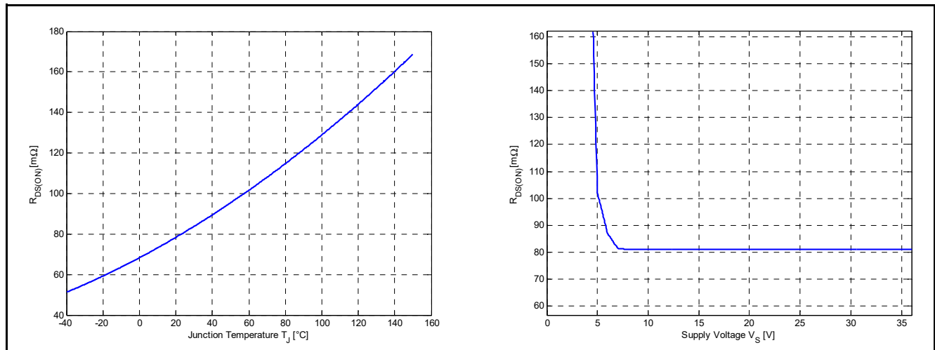
Figure 8 Typical ON-State Resistance
