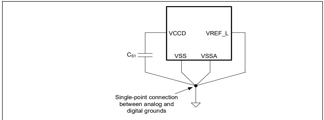
Figure 26-2 Smoothing capacitor
