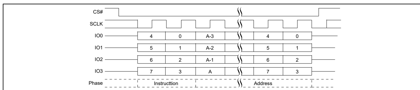
Figure 82 EES QPI mode command sequence [56]
