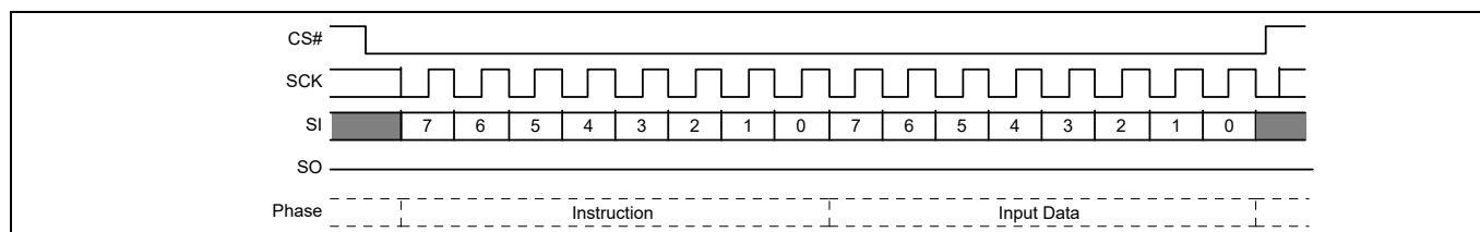
Figure 55 Write VDLR (WVDLR) command sequence
