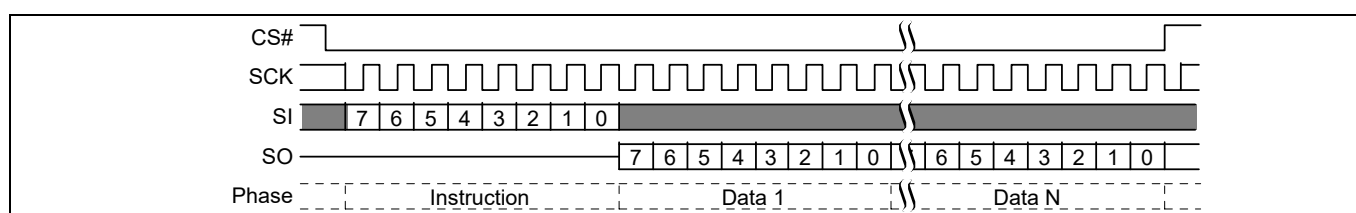
Figure 41 Read Identification (RDID) command sequence
