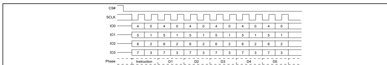
Figure 43 Read Quad Identification (RDQID) command sequence
