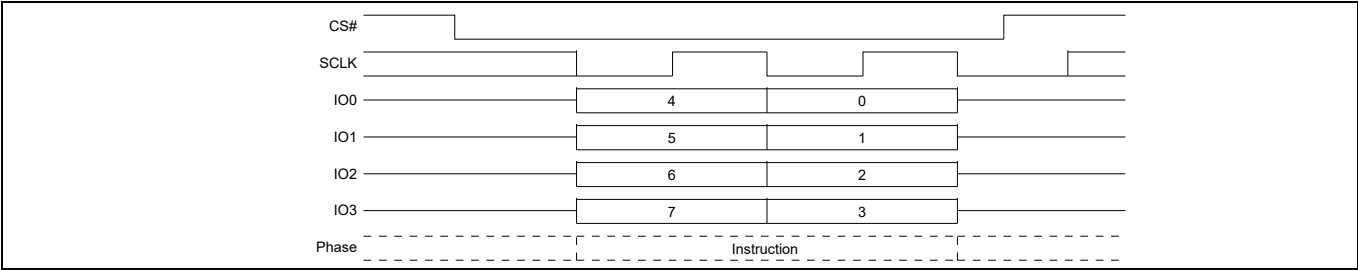
Figure 49 Write Disable (WRDI) command sequence QPI mode
