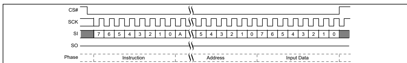
Figure 91 DYBWR command sequence [59, 60]
