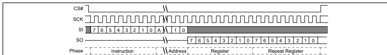
Figure 89 DYBRD command sequence [57, 58]
