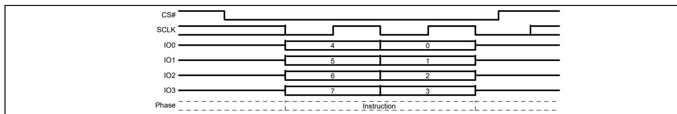
Figure 101 Software Reset command sequence QPI mode
