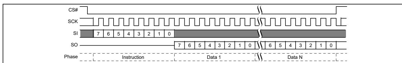
Figure 98 Password Read command sequence
