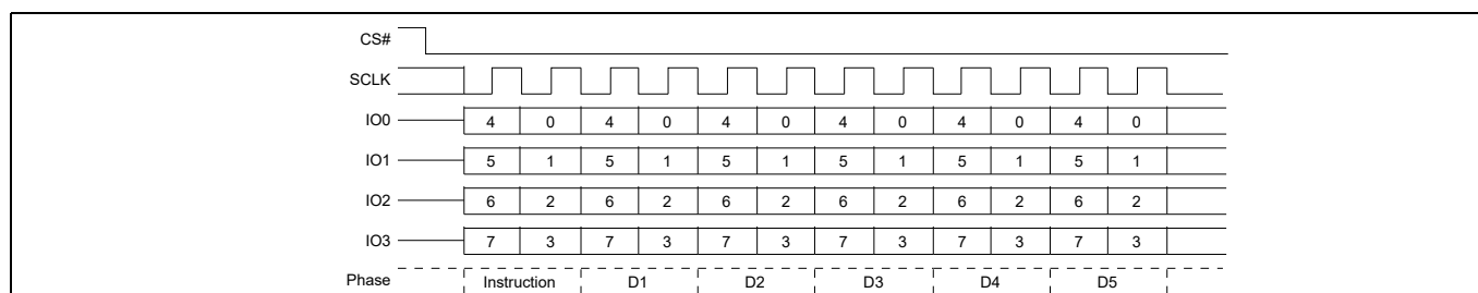
Figure 42 Read Identification (RDID) QPI mode command
