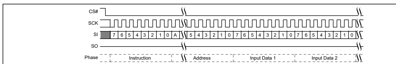
Figure 73 Page Program (PP 02h or 4PP 12h) command sequence [51]
