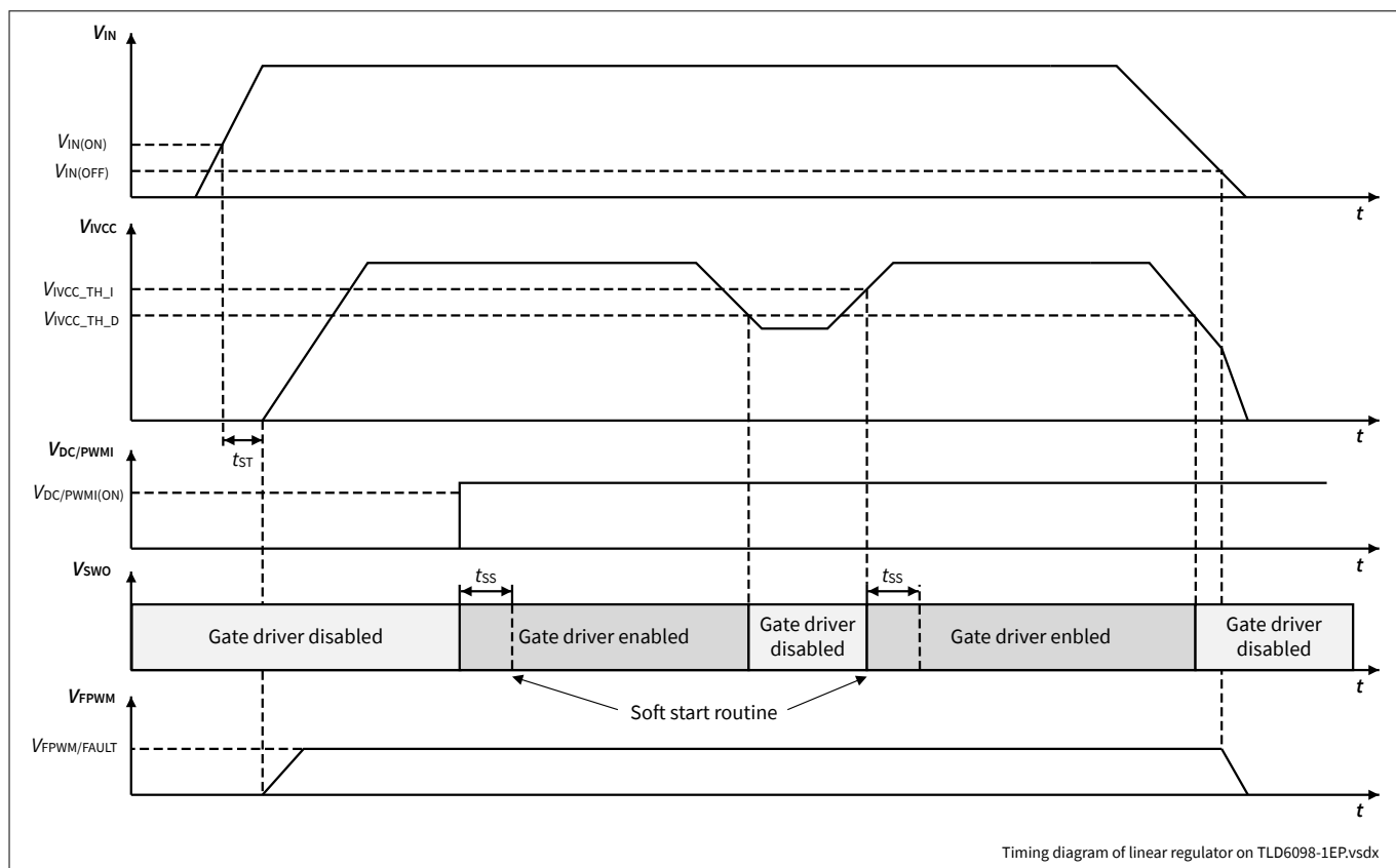
Figure 8 Thresholds and timing diagram related to the linear regulator
