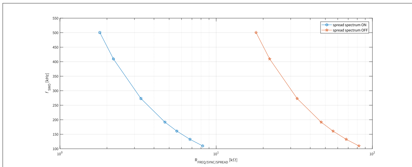
Figure 10 Switching frequency versus R_{\text{FREQ/SYNC/SPREAD}}
